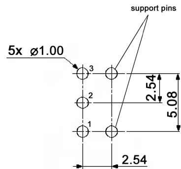
P.C.B. MOUNTING HOLE DIMENSIONS (TOP VIEW)
